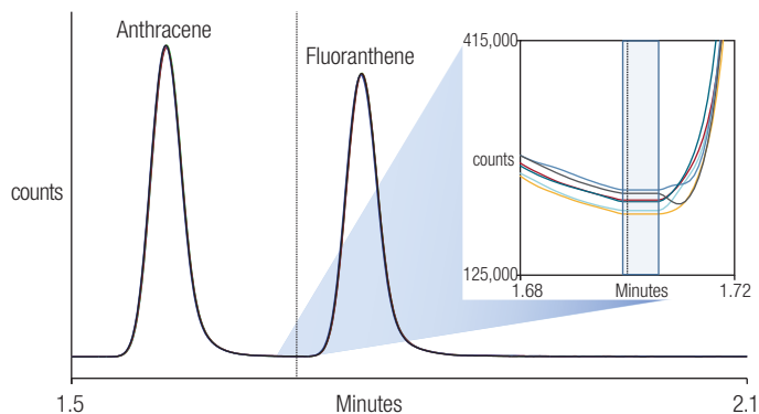
Figure 3. Overlay of six consecutive standard injections with a zoom to baseline level at 1.70 min. Wavelength switching times are extremely short and precise.
