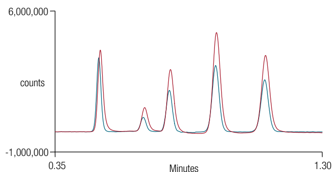
Figure 6. Overlay of two separations obtained on a 2.1 × 50 mm, 3 μm column; detected with a 2 μL micro flow cell (blue) and an 8 μL analytical flow cell (red). The micro flow cell achieves the best resolution, the analytical flow cell provides the best S/N.
