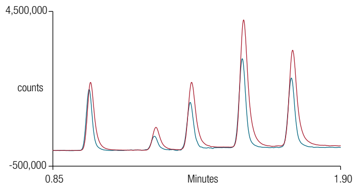
Figure 5. Overlay of two separations obtained on a 3 × 75 mm, 3 μm column with an analytical flow cell (red) and a micro flow cell (blue). The micro flow cell achieves better resolution, the analytical flow cell provides better S/N.
