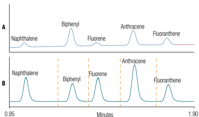
Figure 2. A) UV and B) fluorescence chromatograms of the same sample: All analytes are clearly baseline resolved. The detectors were coupled sequentially, with the UV before the fluorescence. Dotted lines in chromatogram B indicate wavelength switches.
